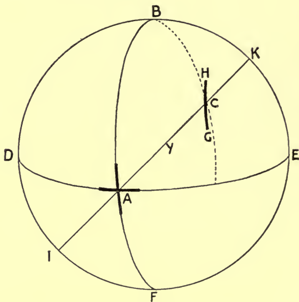
FIG. 191.—Anterior view of the globe showing the position which the vertical arm of the cross assumes when the eyes pass from the primary to a secondary position.
